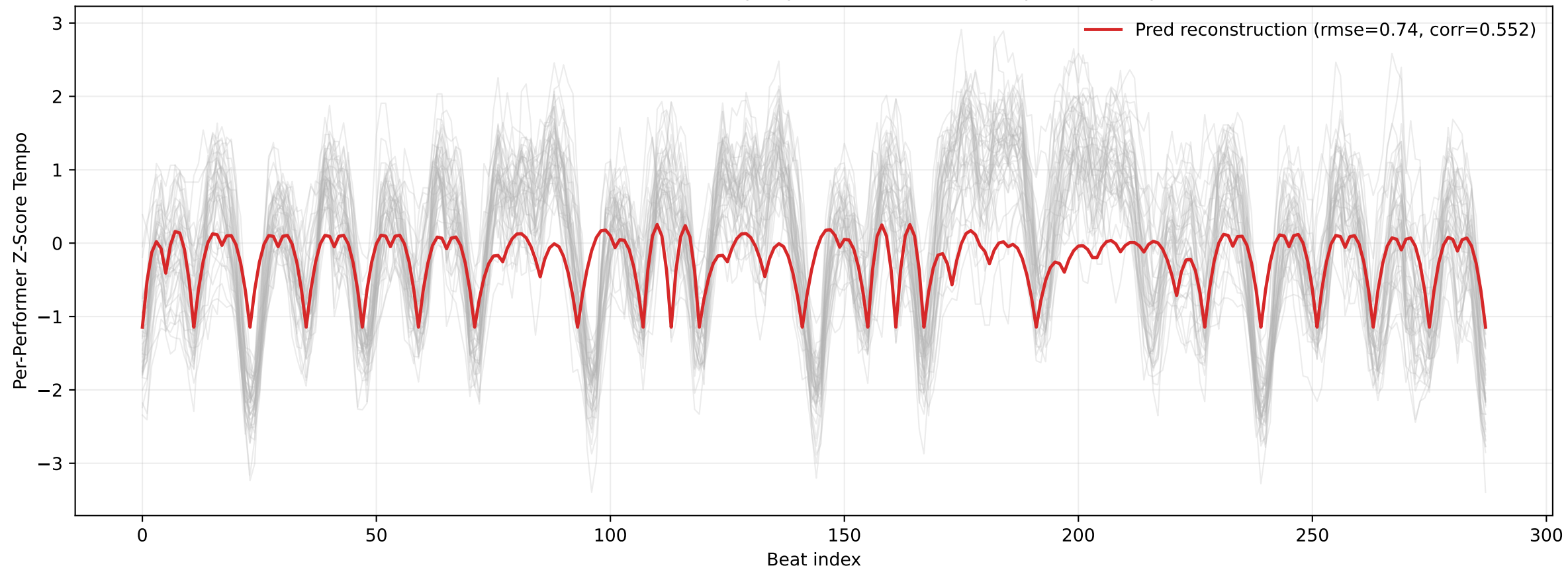
M06-2: Pred reconstruction vs ALL per-performer z-score tempo true tempo curves
